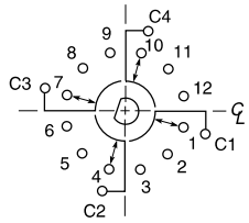
FOUR POLE
