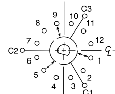
THREE POLE Styles M, MS, H and HS
