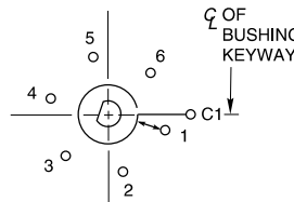
ONE POLE
