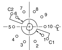
TWO POLE
