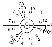
THREE POLE Styles A, D and S
