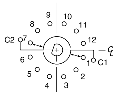
TWO POLE
