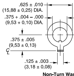
Non-Turn Washer
