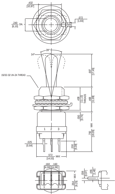
8868 Straight PC Mount
