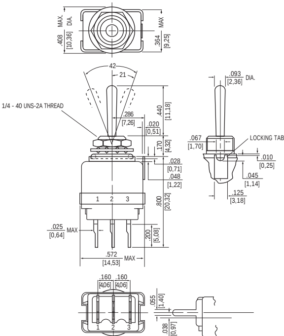
8866 Straight PC Mount
