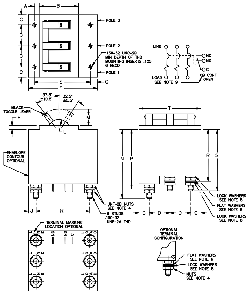
FIGURE 1. Dimensions and configurations (configuration 1).
