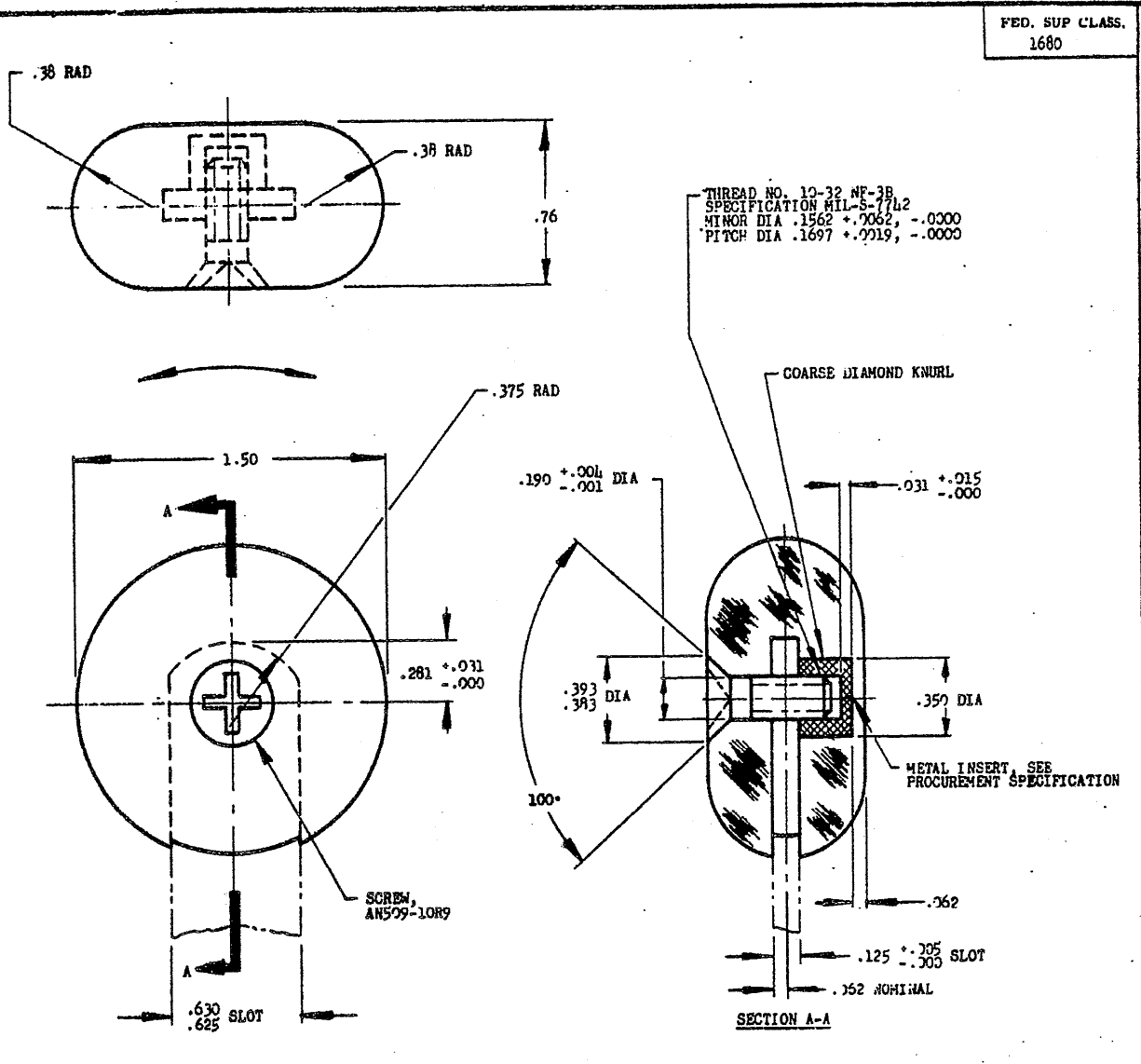
HANDLE, CONTROL, THROTTLE, LARGE
